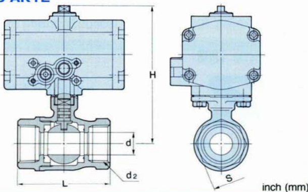
Bronze ball valve with Type C actuator Fig. C-AKTE
