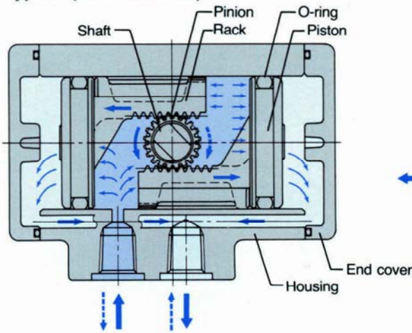
Double-action actuator Type C
